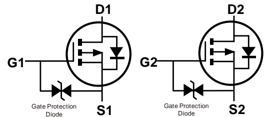
Equivalent Circuit
